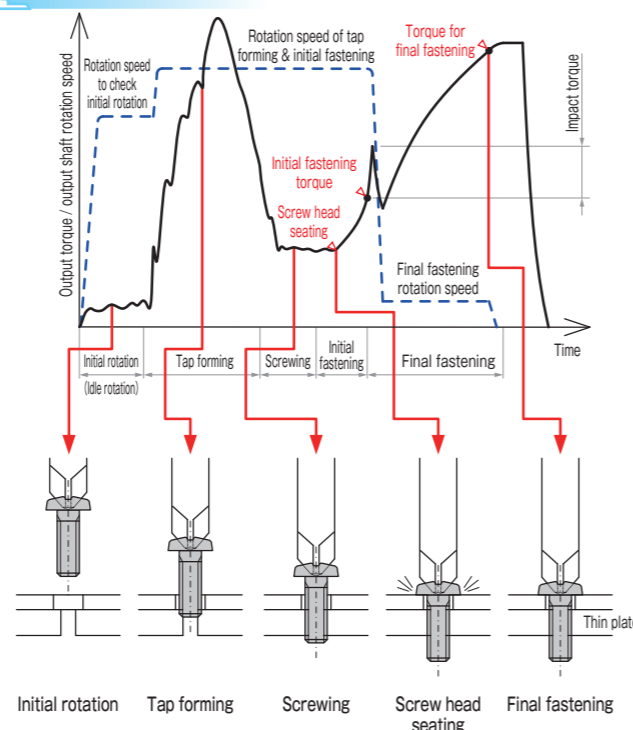
Sample waveform of selftapping screw fastening
