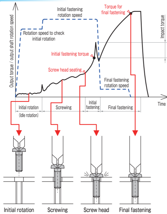
Two-step fastening waveform image
